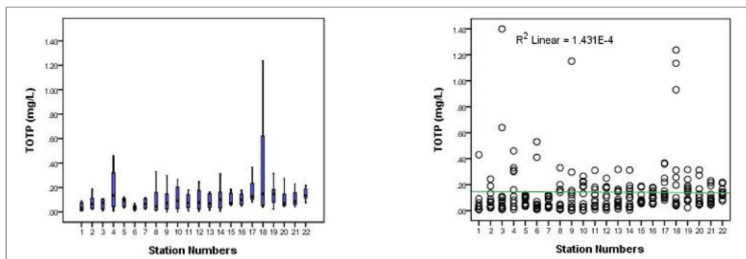
Figure 25: Volumes of Total Phosphorus Concentrations in Urban Wastewater of Main Cities along the Mekong Tributaries
